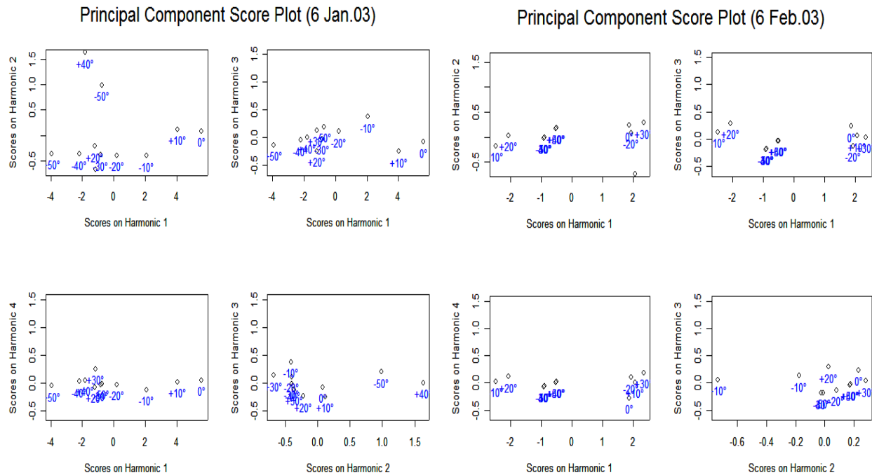
Figure 12. Principal component scores of second fPCA versus first fPCA, third fPCA versus first fPCA, fourth fPCA versus first fPCA and second fPCA versus third fPCA for January and February 2003 data.
