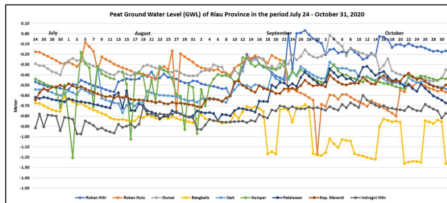
Figure 5. Peat Ground Water Level in Riau Province in the period July 24 - October 31, 2020.
