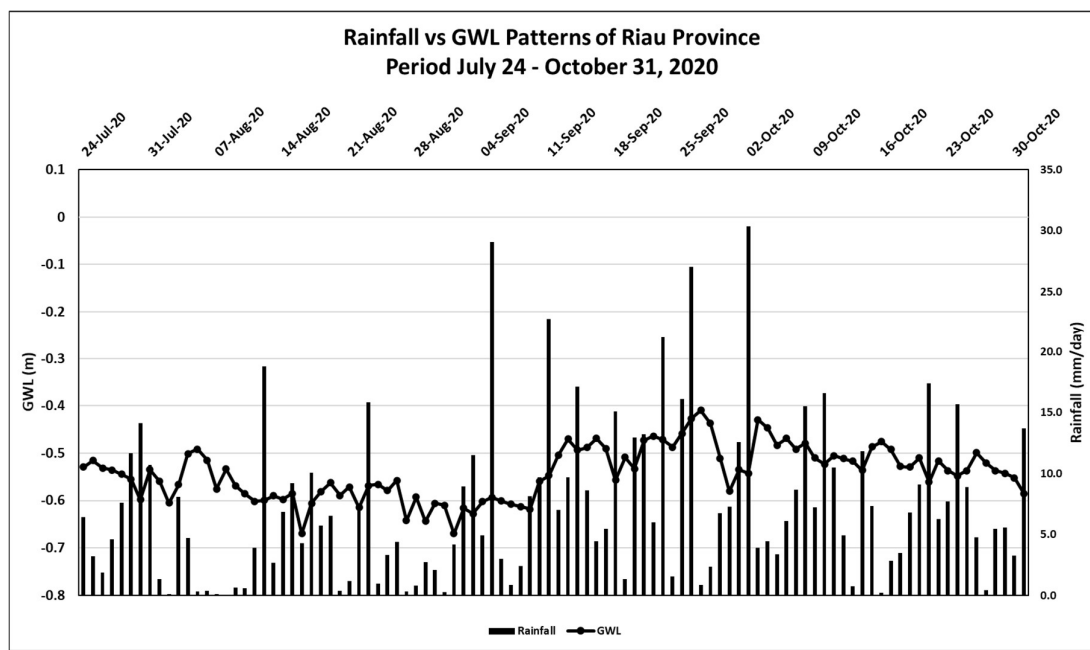
Figure 6. Chart of GWL relationship patterns and daily rainfall in Province Riau, observation period July 24 - October 31, 2020.
