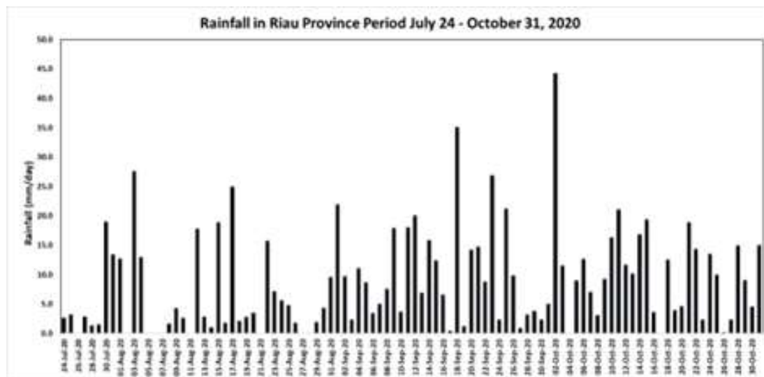
Figure 3. Rainfall chart in Riau Province period July 24 – October 31, 2020.
