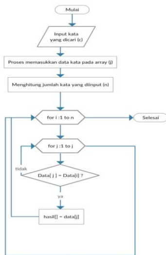
Gambar 6. Flowchart Algoritma Sequential Search
