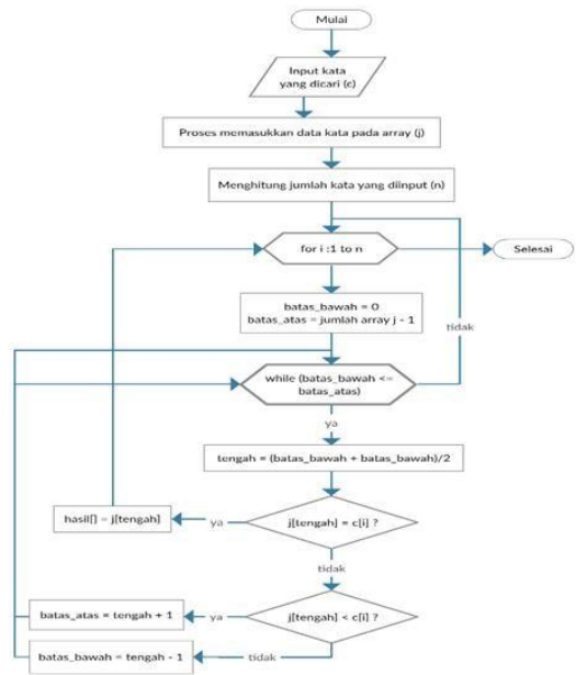
Gambar 7. Flowchart Algoritma Binary Search
