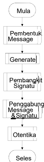
Gambar 6 Flowchart Proses TandaTangan Digital
