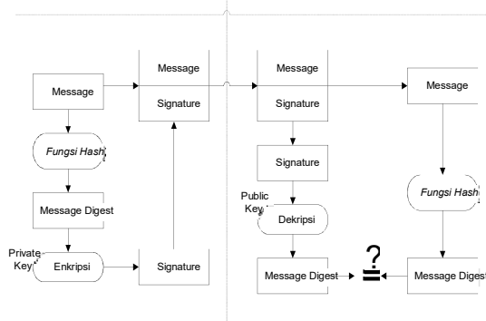
Gambar 5 Gambar Umum Sistem RSA Digital Signature
