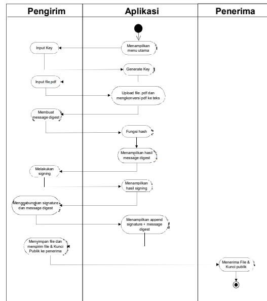
Gambar 12 Activity Diagram Digital Signature
