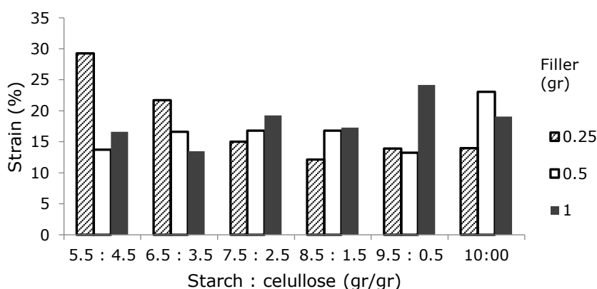
Figure 2. Effect of Starch: Cellulose Ratio(g/g) and Filler Against The Strain of Bioplastics
