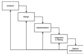
Gambar 1. Metode Waterfall
