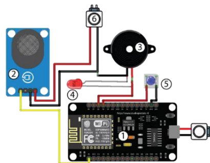
Figure 3. The hardware circuit design
