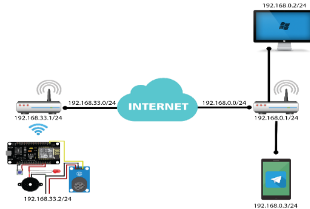
Figure 2. Network design
