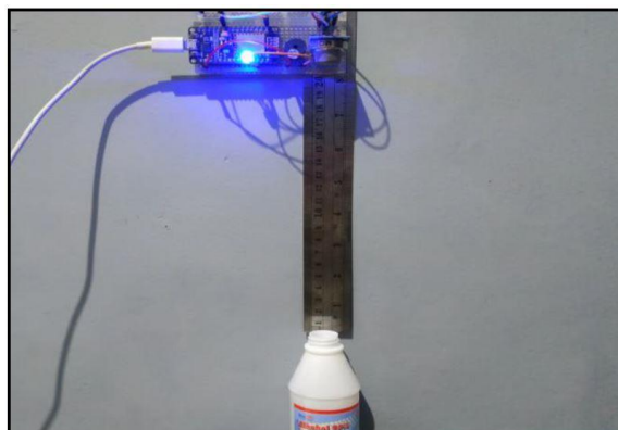
Figure 14. Experimental scenario on evaporation of alcohol gas
