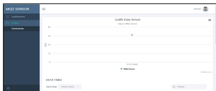
Figure 7. Main menu
