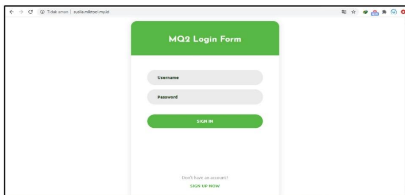
Figure 6. Form login
