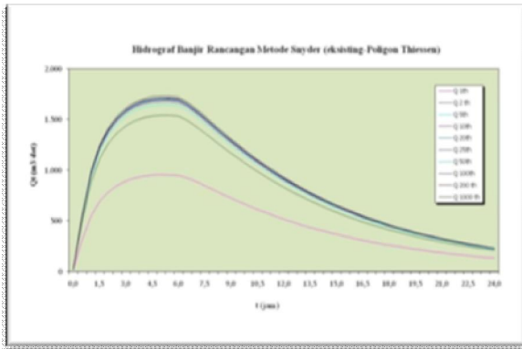
Gambar 3.3 hidrograf banjir rancangan HSS Snyder (Eksisting-Poligon Thiessen)
