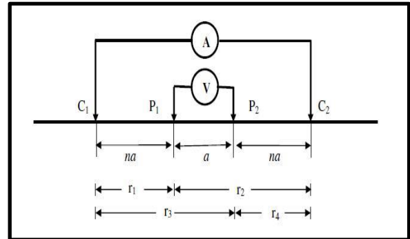
Gambar 5 Konfigurasi Wenner-Schlumberger
