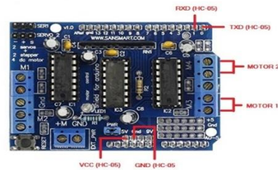
Gambar 3.5 : Motor Shield Arduino L293D
