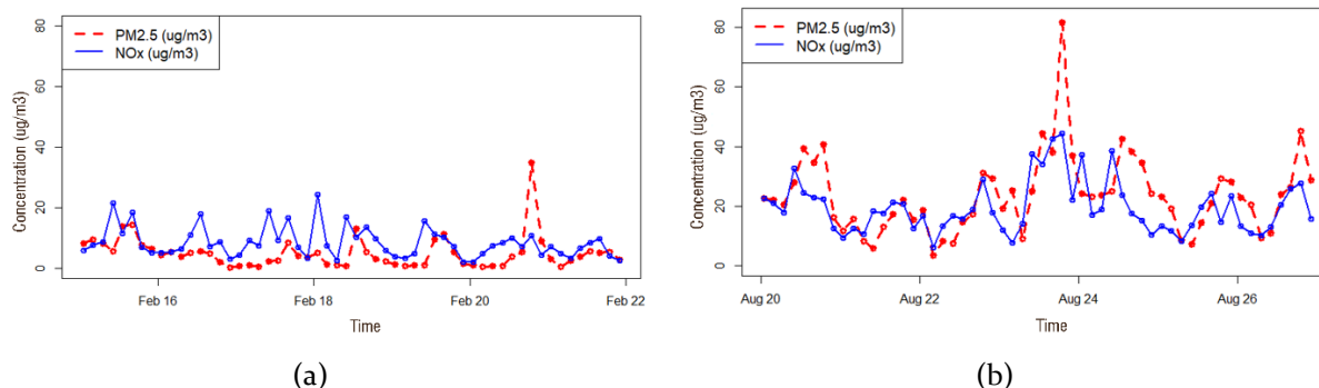
Figure 8. Fluctuations in PM 2.5 and NO x concentrations (a) high rainfall (b) low rainfall in 2020
