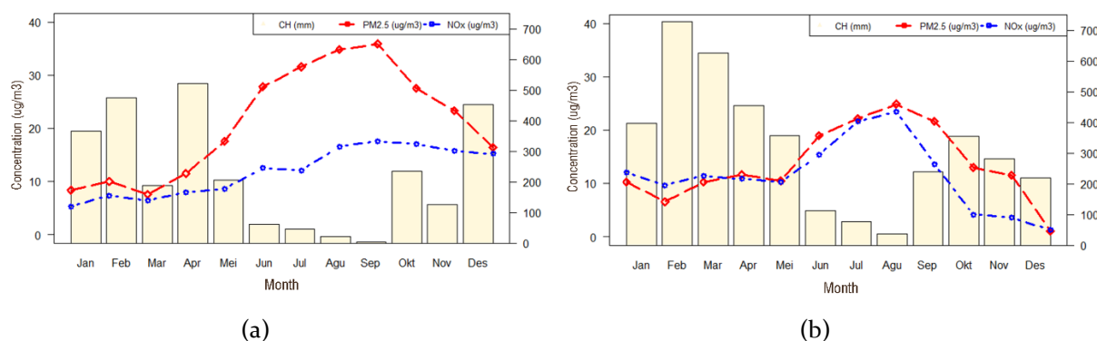
Figure 9. Monthly fluctuations of PM 2.5 concentration, NO x concentration, and rainfall (a) in 2019 (b) in 2020 in Puncak Bogor
