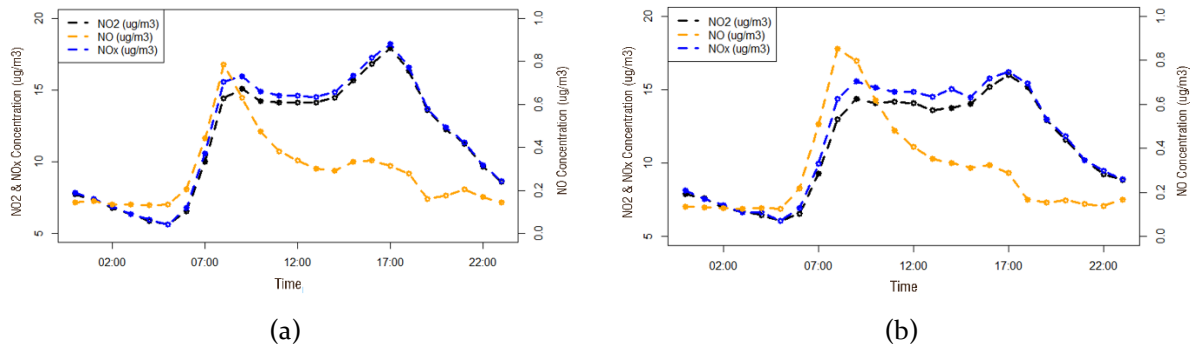
Figure 3. Diurnal average concentrations of NO 2 , NO, and NO x (a) in 2019 (b) in 2020
