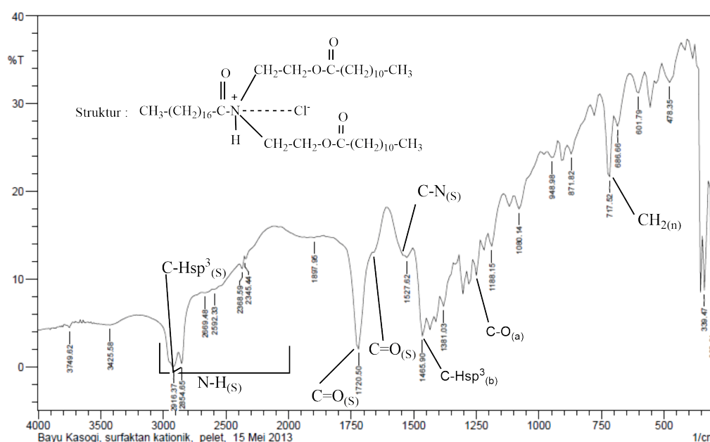
Figure 6. FT-IR Spectrum of Cationic Surfactant N, N-(2-Laurate-Ethyl) Stearamidium Chloride
