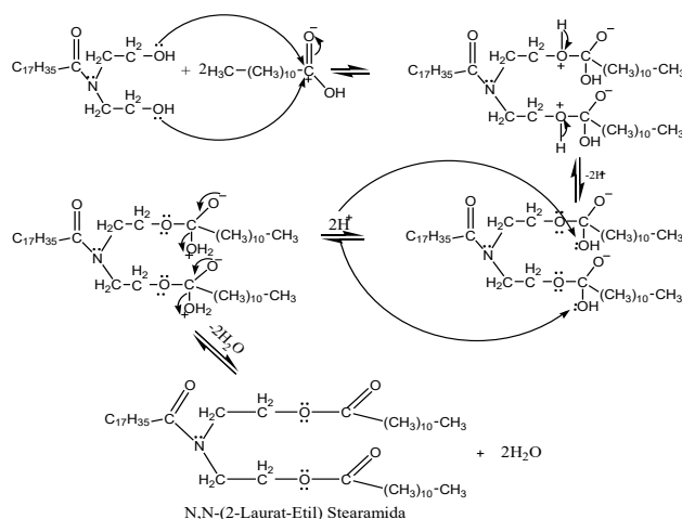
Figure 3. Alkanolamide Esters Formation Reaction Mechanism
