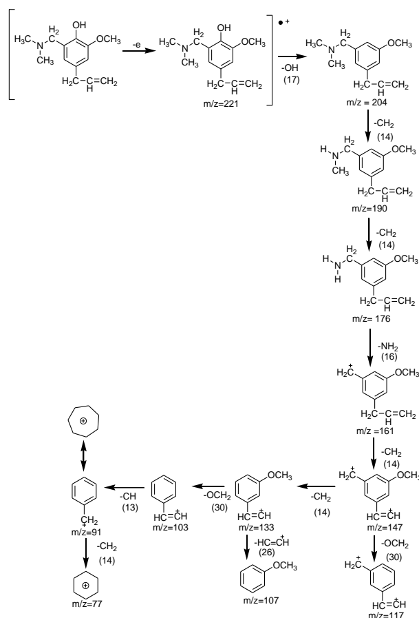
Figure 4.9 Fragmentation pattern of 4-allyl-6-(dimethylamino) methyl-2-methoxy phenol compound
