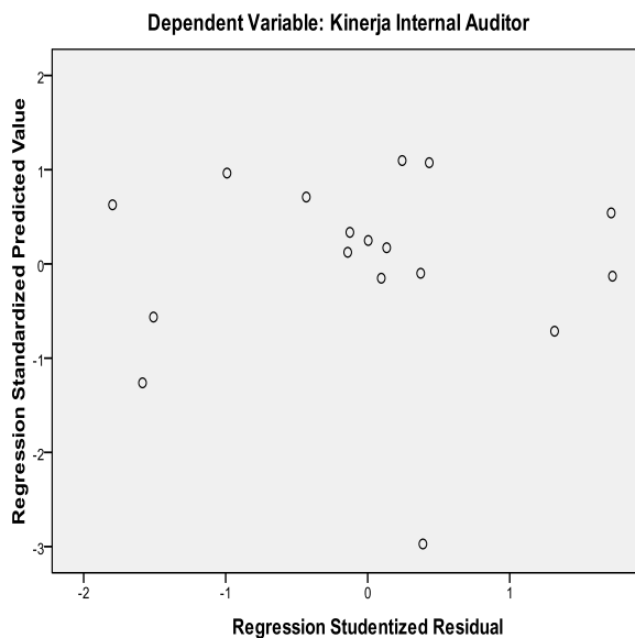
Scatterplot
