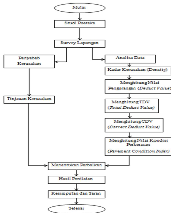
Gambar 2 Flowchart Penelitian
