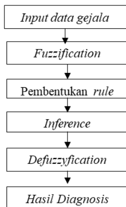
Gambar 2. Mekanisme Fuzzy Tsukamoto
