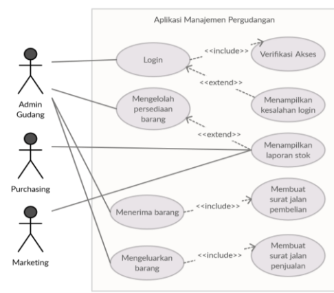
case Diagram
