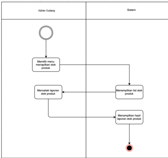
Gambar 5: Activity Diagram Laporan Stok
