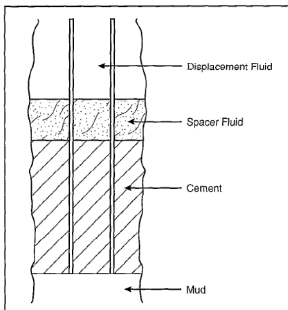
Gambar 2. Balance Plug
