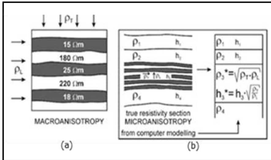
Gambar 2. Geolistrik anisotropi (Anderson, dkk. 1994)
