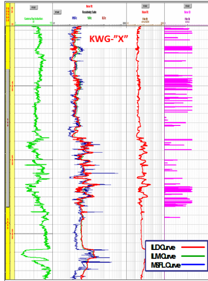
Gambar 6. log resistivitas Sumur KWG “X”
