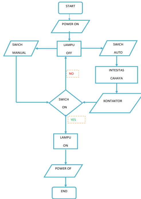
Gambar 3. Flowchart
