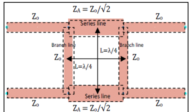
Gambar 1. Rancangan microstrip branch line coupler
