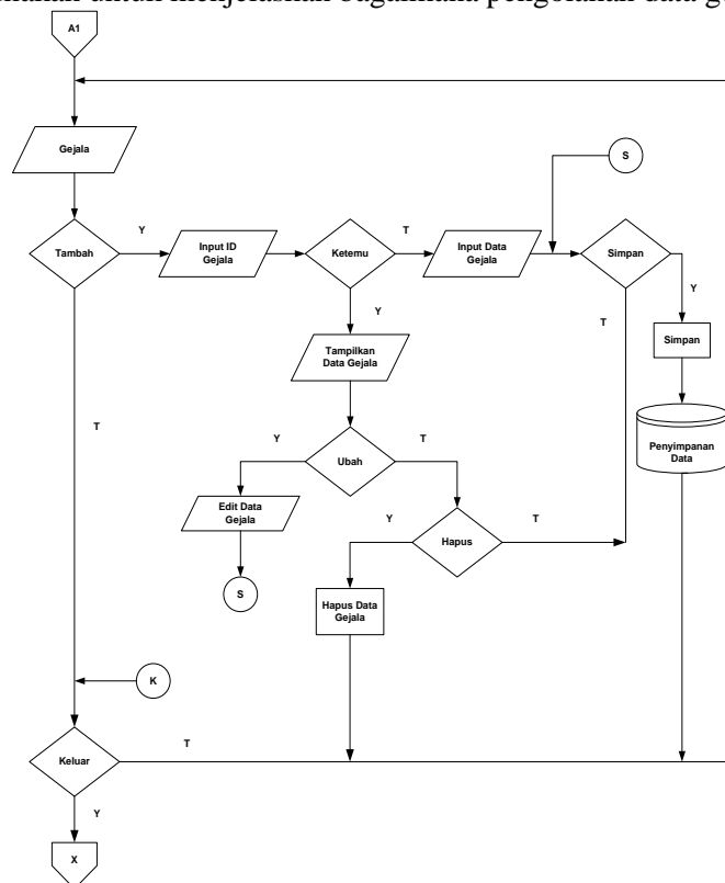
Gambar 5. Flowchart Gejala
