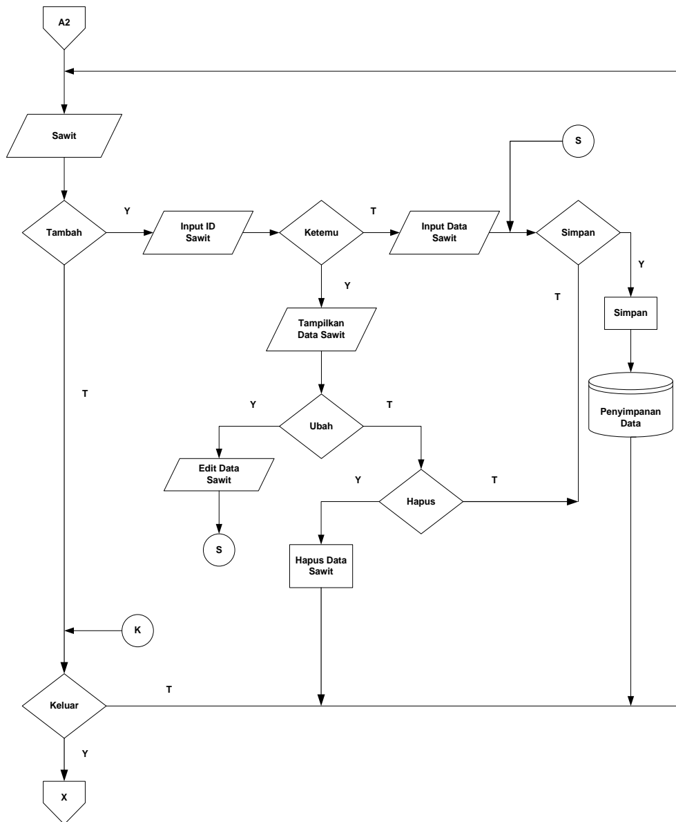
Gambar 6 Flowchart Sawit
