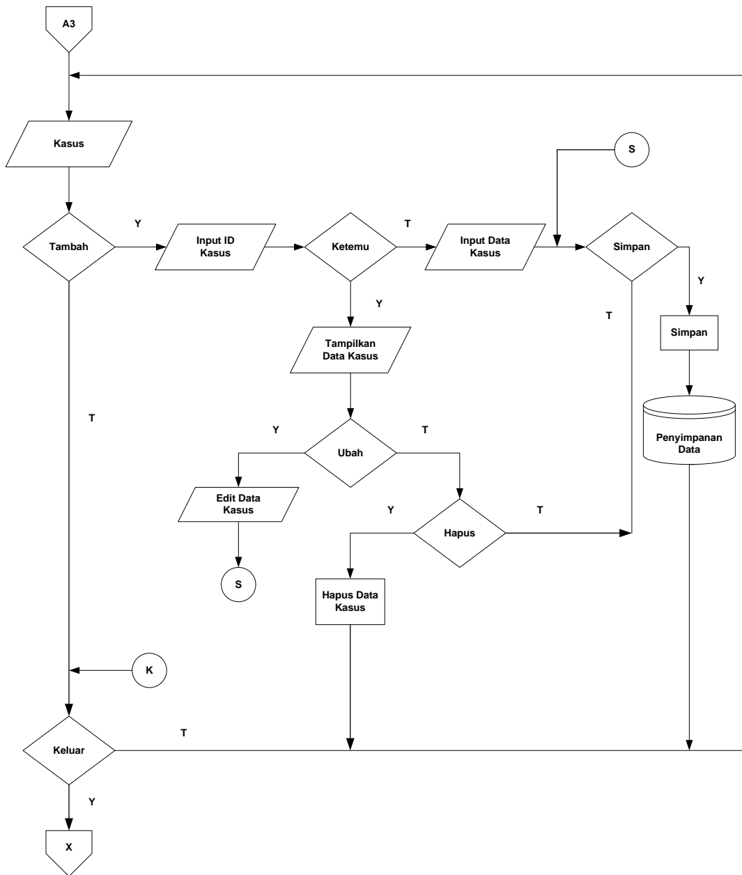
Gambar 7. Flowchart Kasus
