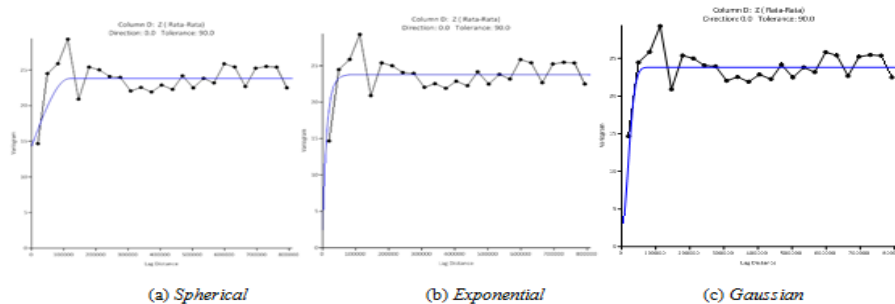
Gambar 2. (a) Hasil Plot Model Spherical (b) Hasil Plot Model Exponential (c) Hasil Plot Model Gaussian
