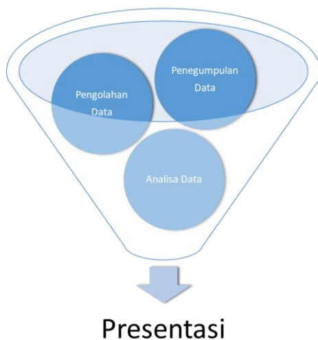
Gambar 1. Metode NIST
