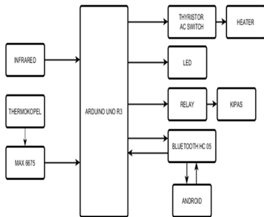
Gambar 2. Diagram Blok
