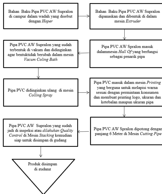
Gambar. 4. Process Diagram Pipa PVC AW 4 Supralon
