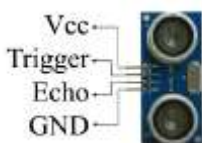
Gambar 1 Sensor Ultrasonik [5]
