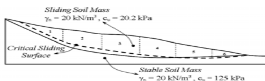
Gambar 5. Potongan irisan lereng (Sumber: Mehmet Rifat Kahyaoglu et all. 2009. Determination of Lateral Loads on Slope Stabilizing Pile)
