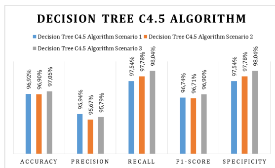
Figure 24. Decision Tree Graph C4.5 Algorithm
