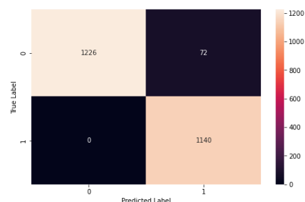
Figure 12. Graph of Confusion Matrix Scenario 1
