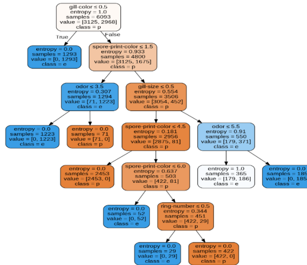
Figure 22. Decision Tree Results Algorithm C5.0 Scenario 2
