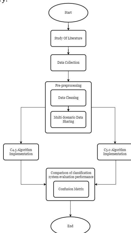
Figure 1. Research Flowchart
