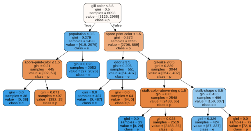
Figure 19. Decision Tree Results Algorithm C4.5 Scenario 2
