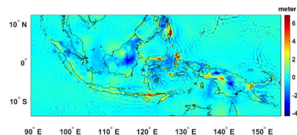
Figure 6. Differences between EGM2008 and EGM96.
