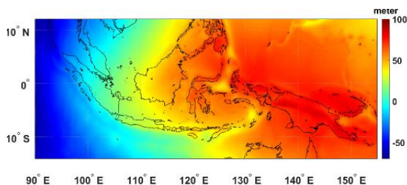
Figure 4. Geoid undulation as calculated using EGM2008.
