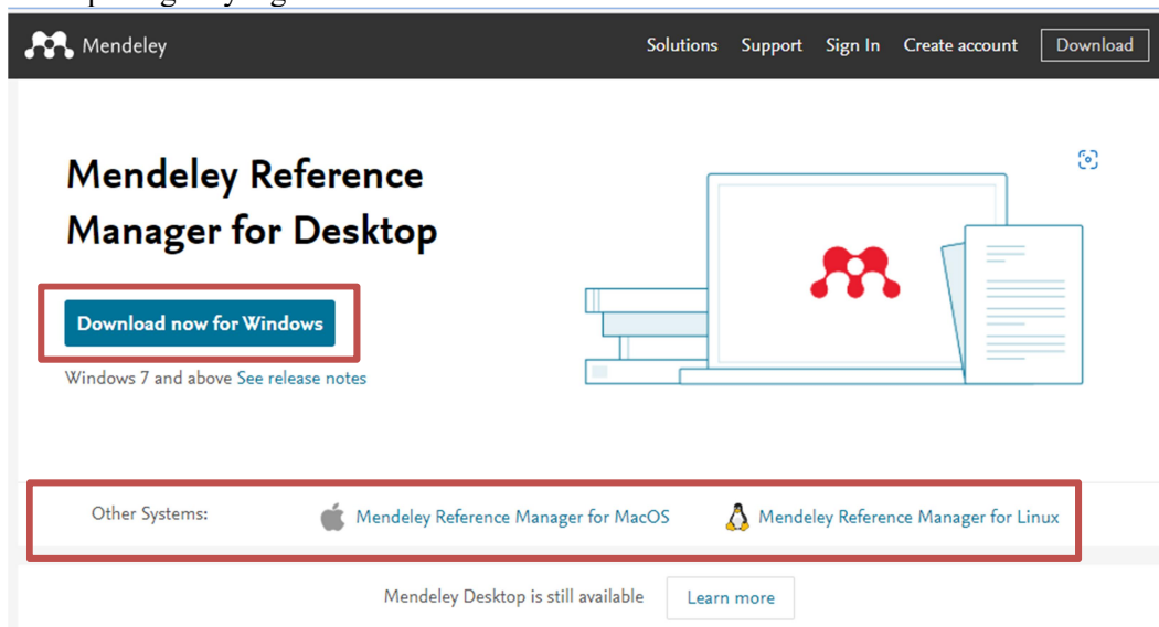
Gambar 4. Download Software
