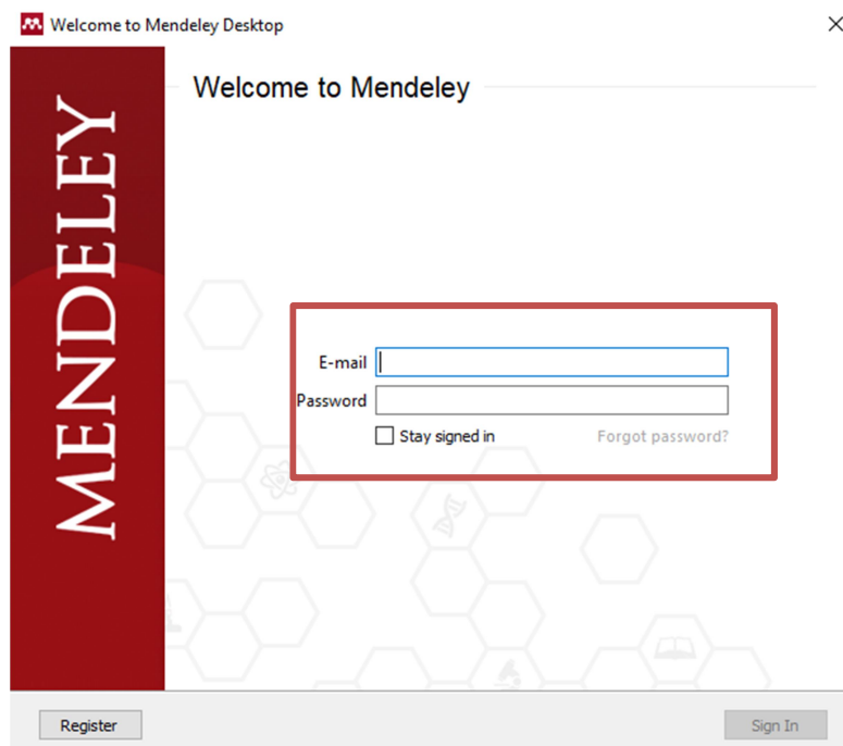
Gambar5. Login Mendeley
