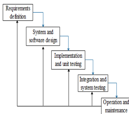
Gambar 1. Metode Waterfall
