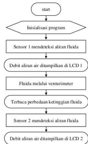
Gambar 2. Diagram Sistem Alat Peraga
