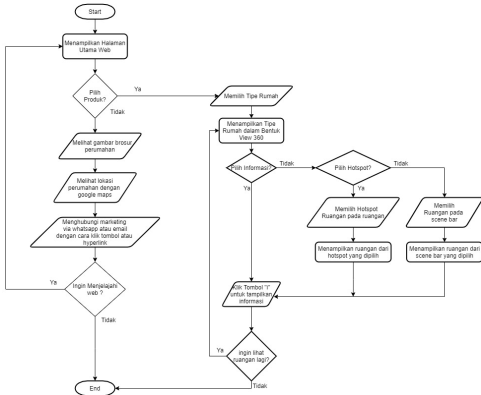
Gambar 3 Flowchart
