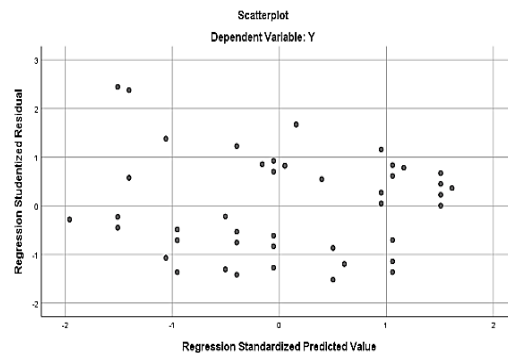
Figure 2. Heteroscedasticity
