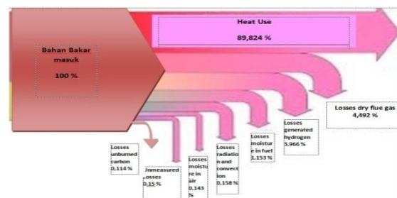
Gambar 3 Diagram sankey
