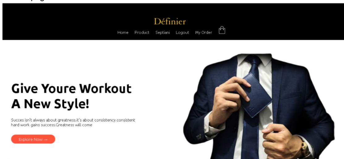
Figure 4. Homepage View
