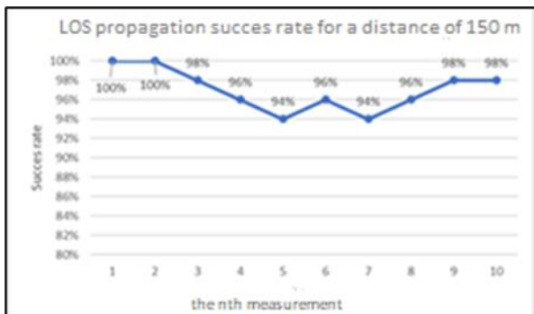
Figure 5. Graph of Success Rate on LOS Propagation Measurement at a 150 m
