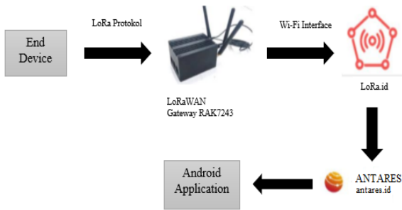
Figure 1. LoRaWAN Communication Architecture
