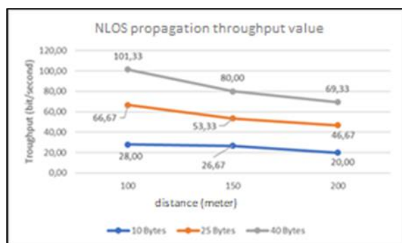
Figure 13. Throughput Graph on NLOS Propagation Measurement
