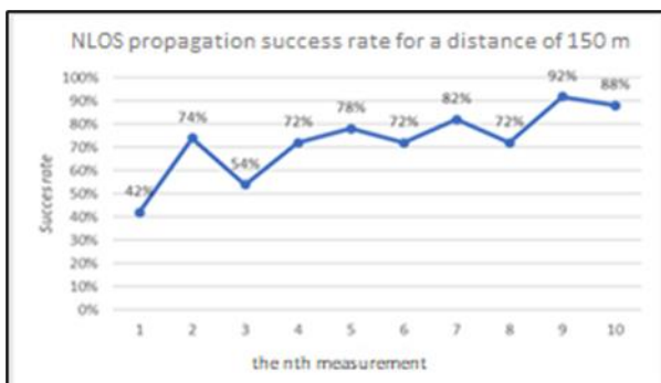
Figure 9. Graph of Success Rate on NLOS Propagation Measurements at a 150 m
