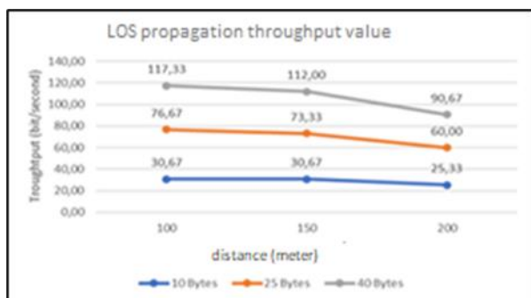
Figure 12. Throughput Graph on LOS Propagation Measurement
