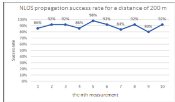
Figure 10. Graph of Success Rate on NLOS Propagation Measurements at a 200 m
