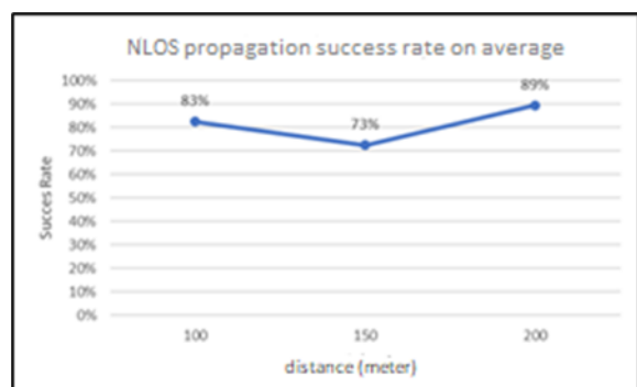
Figure 11. Graph of Average Success Rate on NLOS Propagation Measurements
