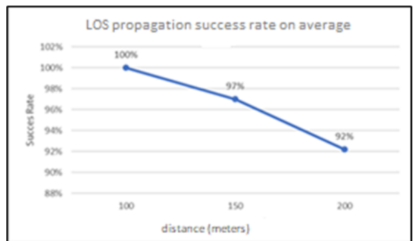
Figure 7. Graph of Average Success Rate on LOS Propagation Measurement
