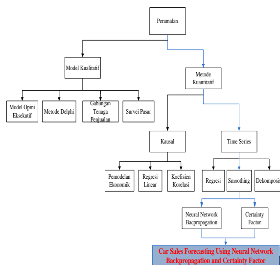
Gambar 3. Flowchart Metodologi Penelitian
