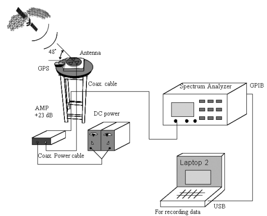
Fig.10. Configuration of the outdoor measurement at roof-top building
