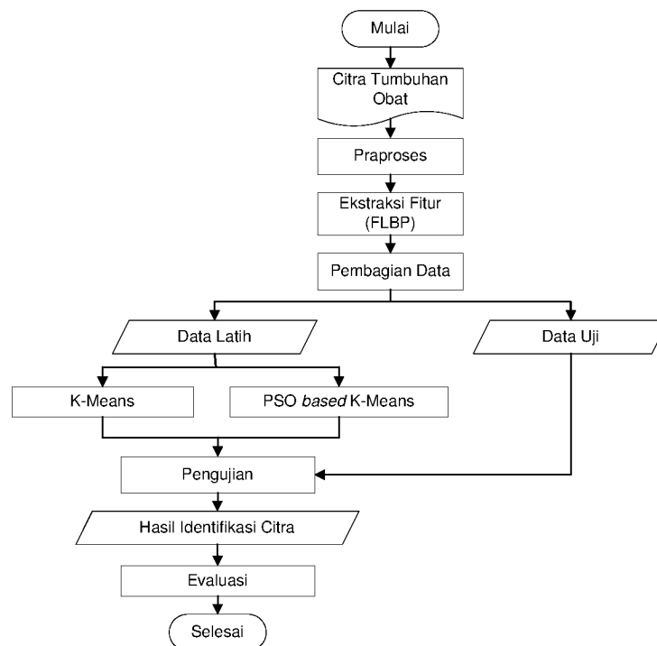
Gambar 1 Metode penelitian
