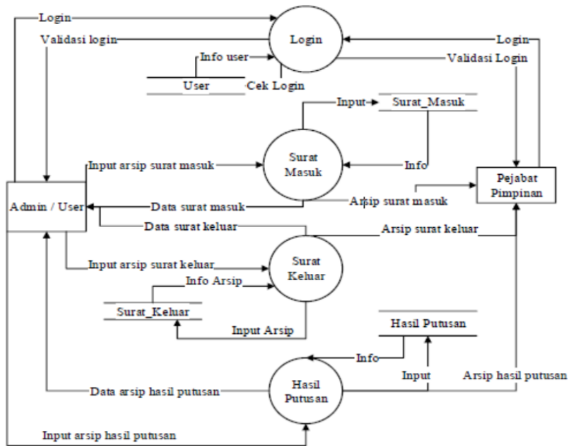
Gambar 2. Data flow diagram (DFD)
