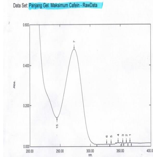
Gambar 1. Kurva Serapan Larutan Baku Kafein ( C = 4,0 \mu\text{g/ml} )
