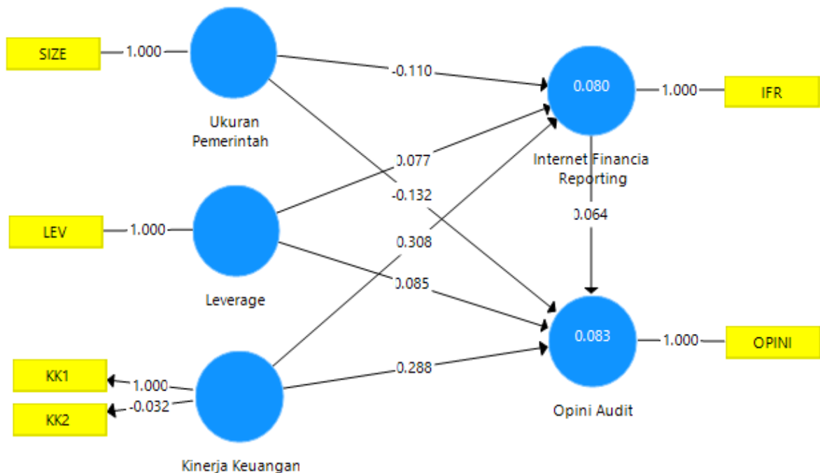
Gambar4.2 Hasil PLSAlgorithmAwal
