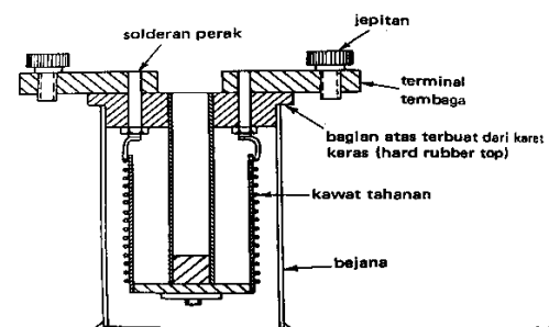
Gambar 5. Penampang Standar Tahanan Dinding Rangkap (Cooper, William D.,1999)
