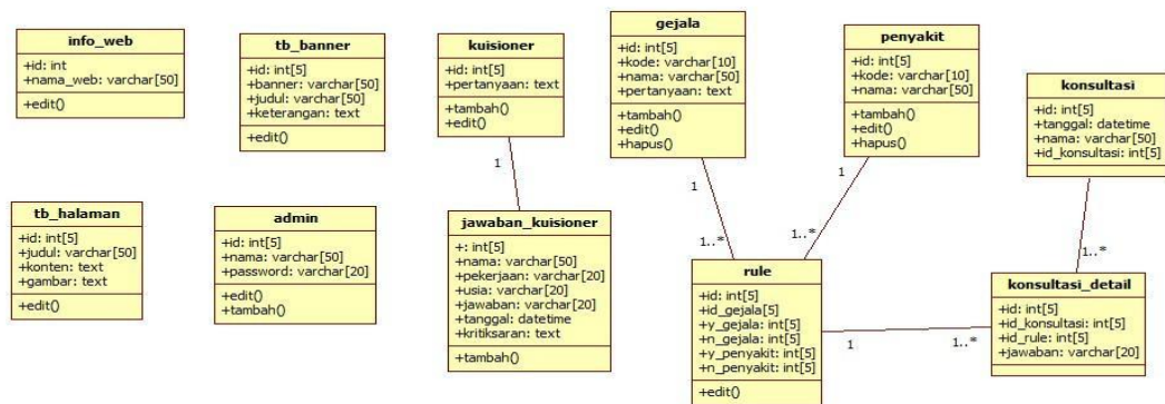
Gambar 1 Class Diagram Sistem Pakar
