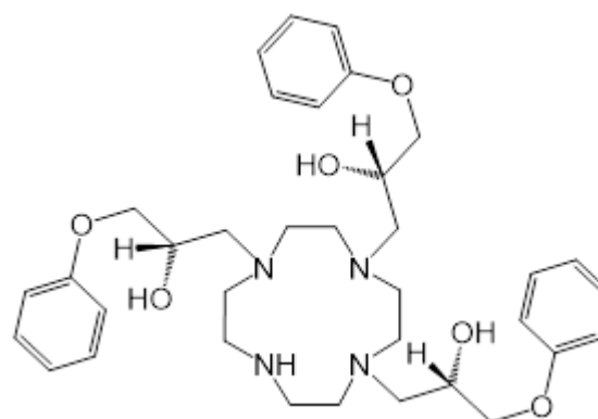
Figure 9. Preparation 1,4,7,10-tris-((2S)-(-)-2-hydroxy-3-phenoxypropyl)-1,4,7,10-tetraazacyclododecane
