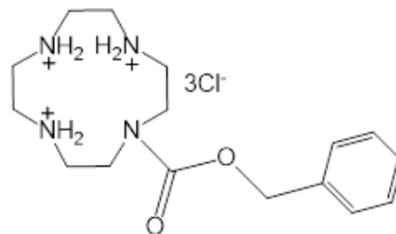
Figure 5. 1-(benzyloxycarbonyl)-1,4,7,10-tetraazadodecane·3HCl·1.5H 2 O, 6
