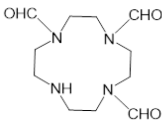
Figure 3. 1,4,7-triformyl-1,4,7,10-tetraazacyclododecane, 4
