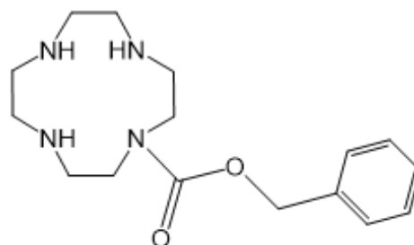
Figure 6. 1-(benzyloxycarbonyl)-1,4,7,10-tetraazacyclododecane, 7
