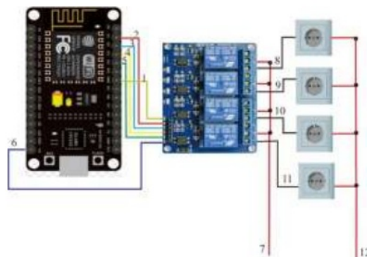
Fig.4. Tool Scheme
