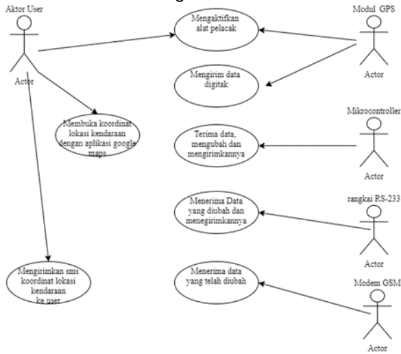
Gambar 4. Usecase Diagram
