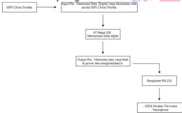
Gambar 5. Activity Diagram
