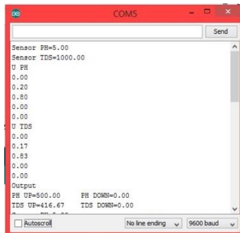
Gambar 7. Hasil Percobaan Fuzzy Logic
