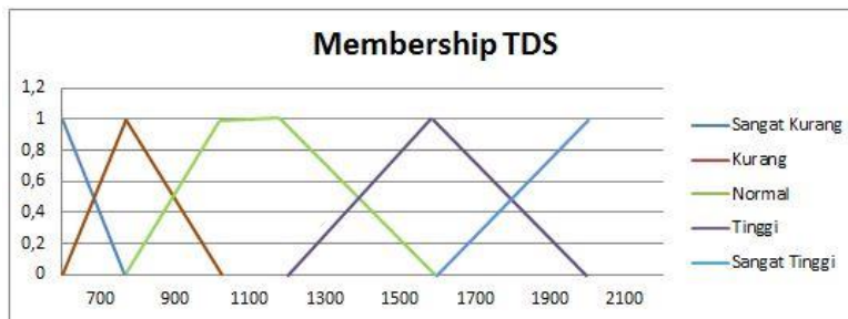
Gambar 6. Membership Function TDS
